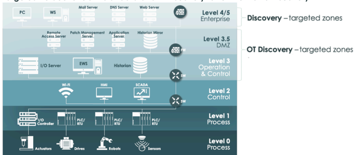
Targeted Purdue levels in standard and IT Discovery for OT Networks Discovery
