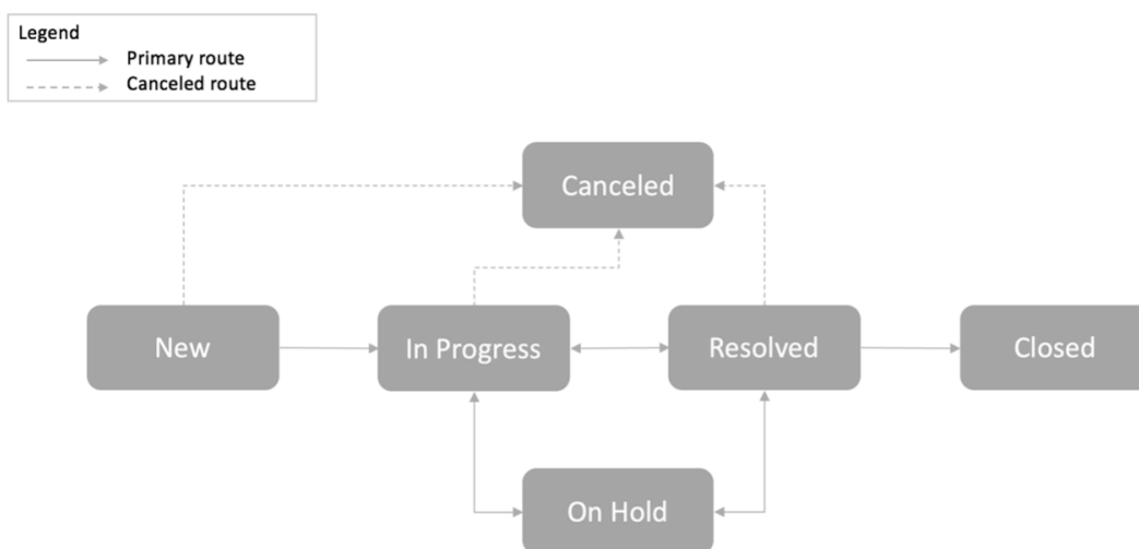
Operational Technology Incident Management process states
